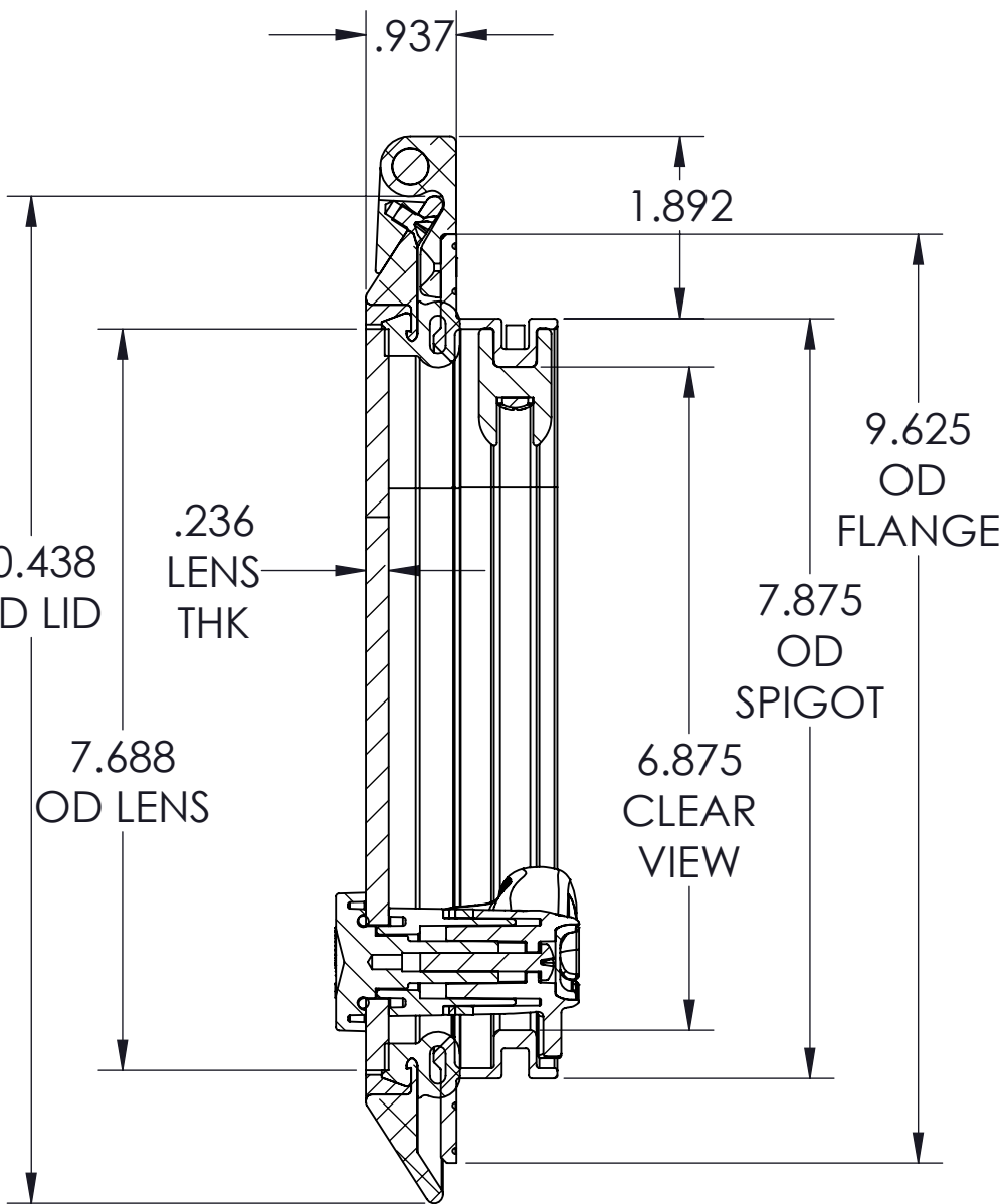
SECTION B-B
